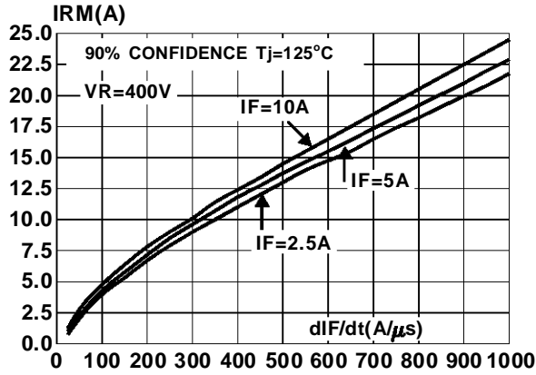
Fig 10 : Peak reverse recovery current versus dI_F/dt
