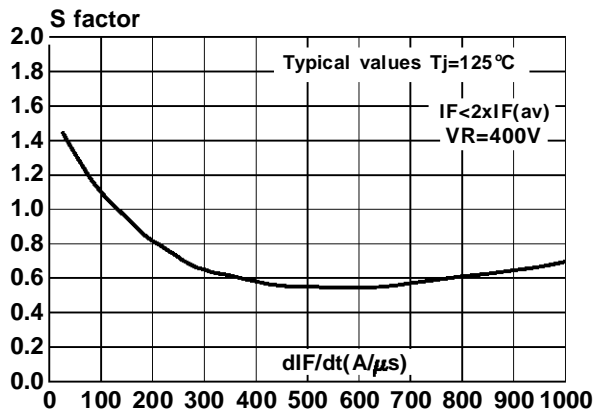
Fig 12 : Softness factor (tb/ta) versus dI_F/dt
