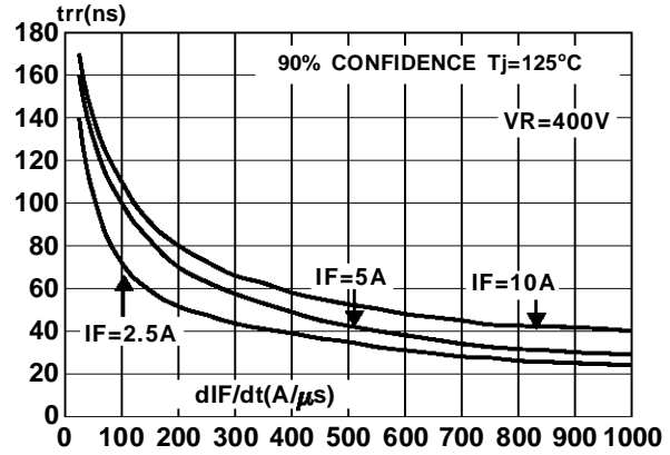
Fig 11 : Reverse recovery time versus dI_F/dt
