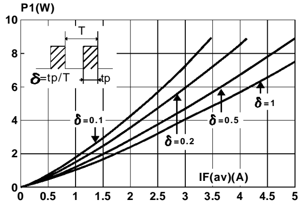
Fig 5 : Conduction losses versus average current
