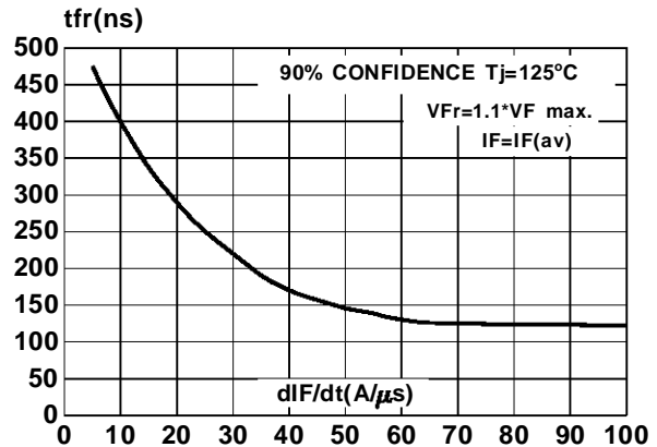
Fig 15 : Forward recovery time versus dI_F/dt
