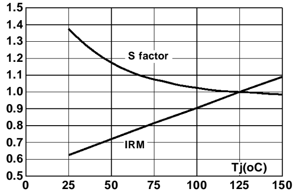
Fig 13 : Relative variation of dynamic parameters versus junction temperature (Reference T_j = 125^\circ C )
