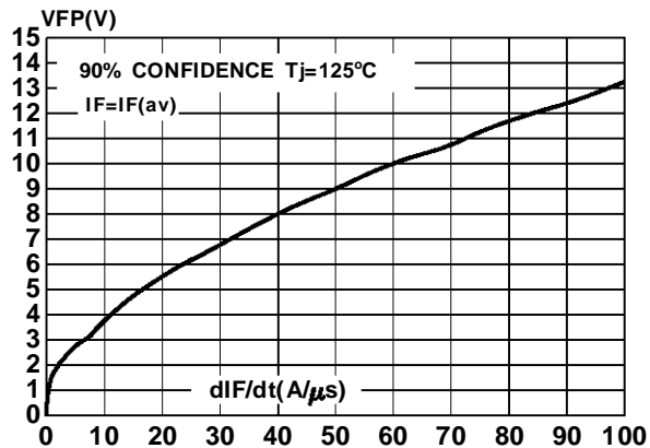
Fig 14 : Transient peak forward voltage versus dI_F/dt
